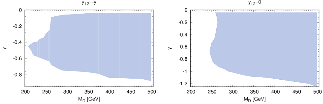
(a) M_D vs y , for \Lambda = 1 TeV and y_{12} = -y . (b) M_D vs y , for \Lambda = 1 TeV and y_{12} = 0 .
