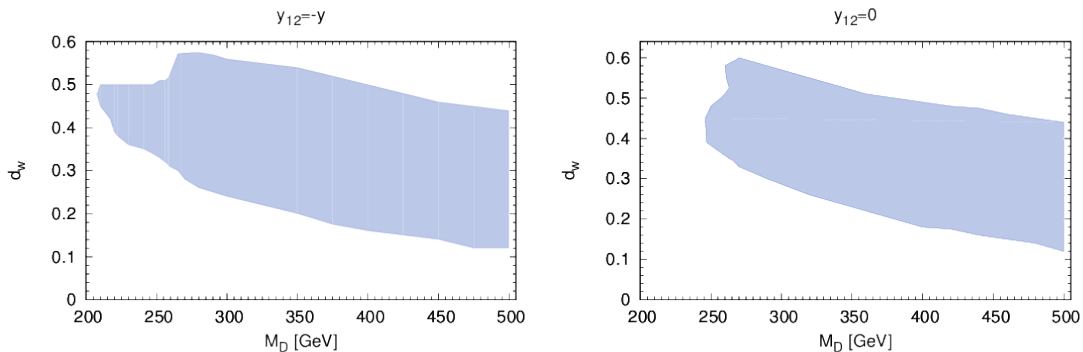
(a) M_D vs d_W , for \Lambda = 1 TeV and y_{12} = -y . (b) M_D vs d_W , for \Lambda = 1 TeV and y_{12} = 0 .
