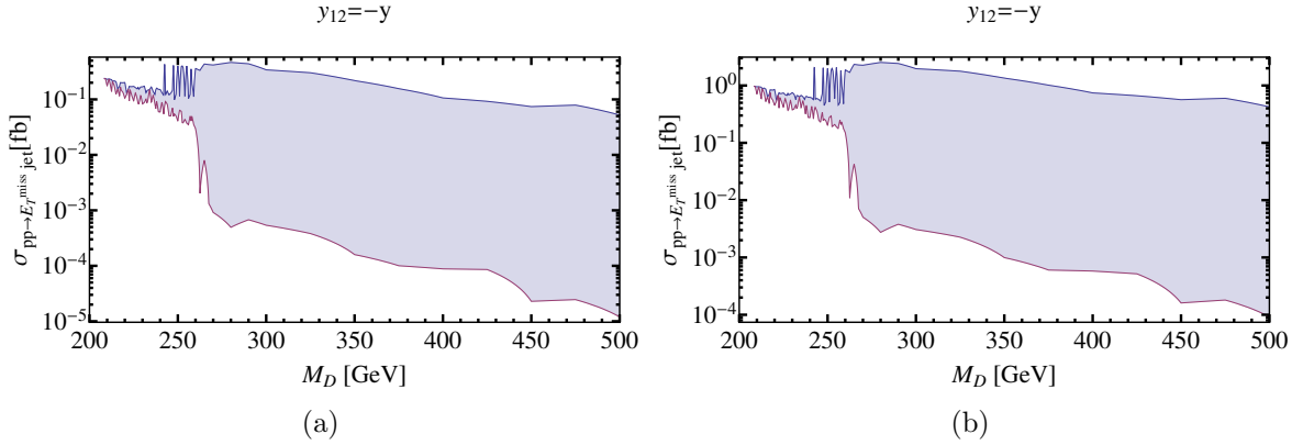
Figure 4.22: As in Fig. 4.21 for the mono-jet channel with (a) \sqrt{\hat{s}} = 8 TeV and (b) \sqrt{\hat{s}} = 13 TeV.
