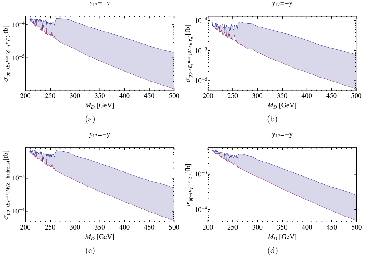
Figure 4.21: The cross sections for the (a) mono-Z, (b) mono-W, (c) hadronically decaying Z/W and (d) the dijet processes at \sqrt{\hat{s}} = 8 TeV versus the doublet-mass parameter M_D , while all the other parameters run freely and for y_{12} = -y . The other case with y_{12} = 0 gives almost identical results. The “spikes” appeared is a result of varying a random selection of parameters.
