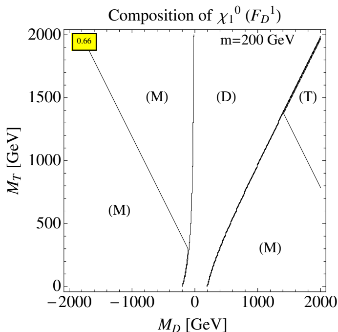
Figure 3.3: The composition of the WIMP in terms of (D)oublet, (T)riplet and (M)ixed states following the definition given in the paragraph below eq. (3.52), on a M_D vs. M_T plane and for fixed (common) Yukawa coupling, Y = m/v \simeq 200/174 \simeq 1.15 .
