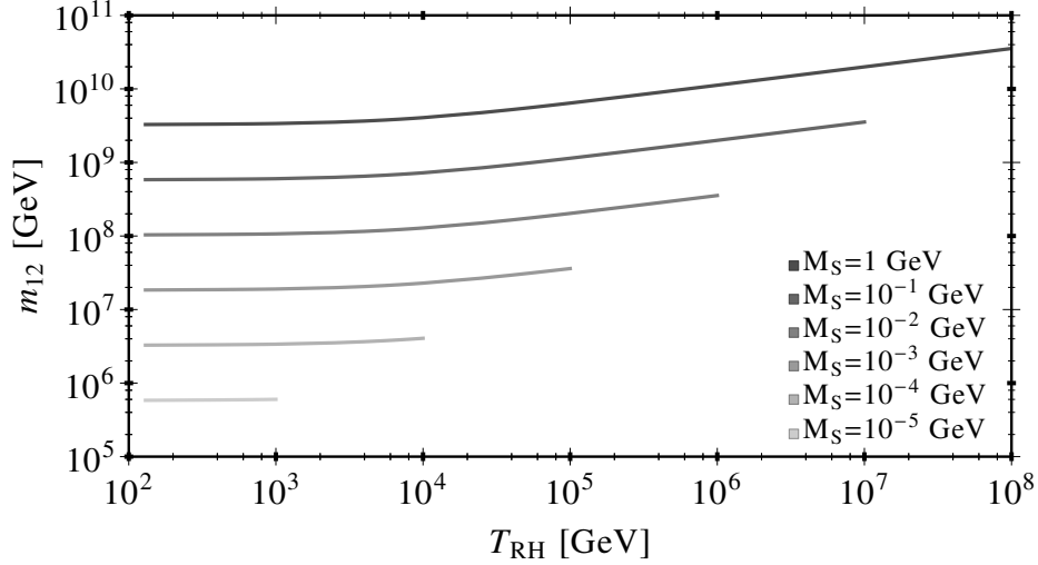
Figure 5.3: T_{\text{RH}} versus m_{12} for r = M_D/m_{12} = 10^{-2} , t_\beta = 1 and several RLDM masses M_S .
