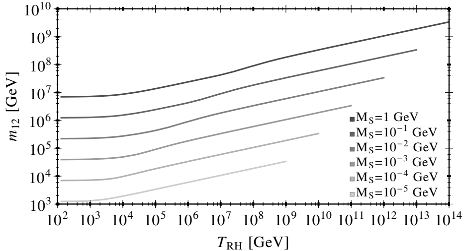
Figure 5.4: The same as in Figure 5.4, but for r = M_D/m_{12} = 10^5 .
