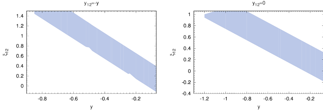
(a) y vs \xi_{12} , for \Lambda = 1 TeV and y_{12} = -y . (b) y vs \xi_{12} , for \Lambda = 1 TeV and y_{12} = 0 .
